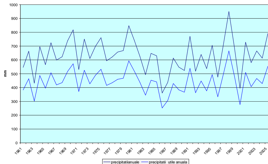
Fig. 1 The annual quantity of precipitations and useful precipitations in Sibiu in the period 1961-2005
